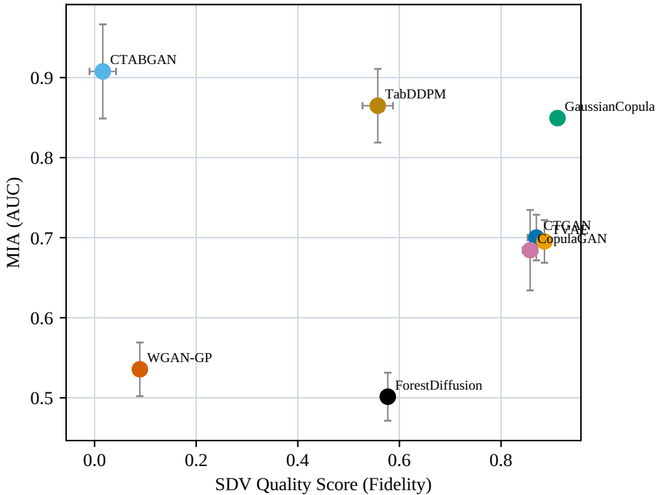
CDC Diabetes: SDV Quality Score (Fidelity) vs MIA (AUC)
